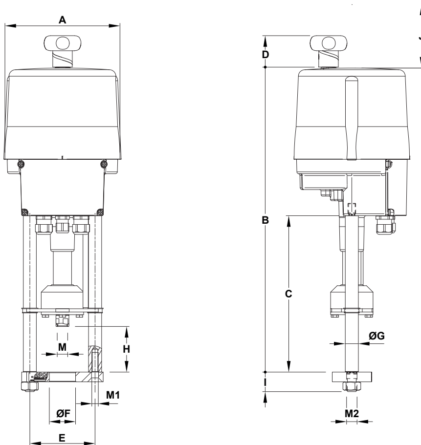
DIMENSIONS (mm)
