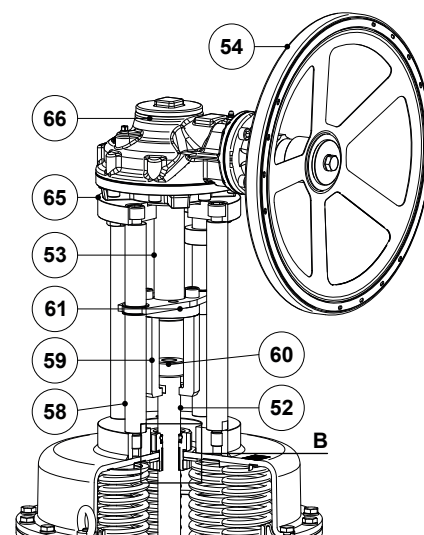
PA80D – PA80T Top mounted handwheel with worm gear
