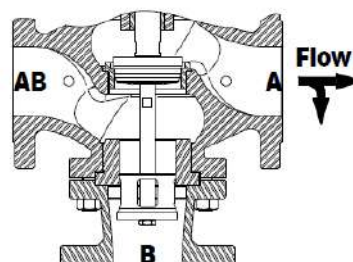
Diverting valve
