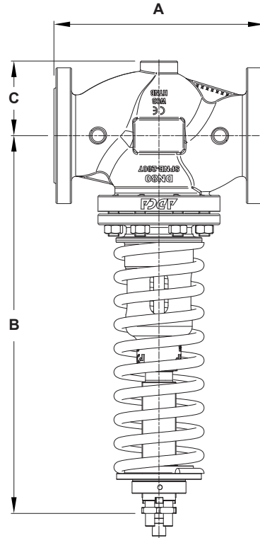
DIMENSIONS – VALVE (mm)
